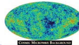
COSMIC MICROWAVE BACKGROUND
