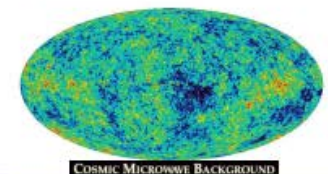
COSMIC MICROWAVE BACKGROUND
